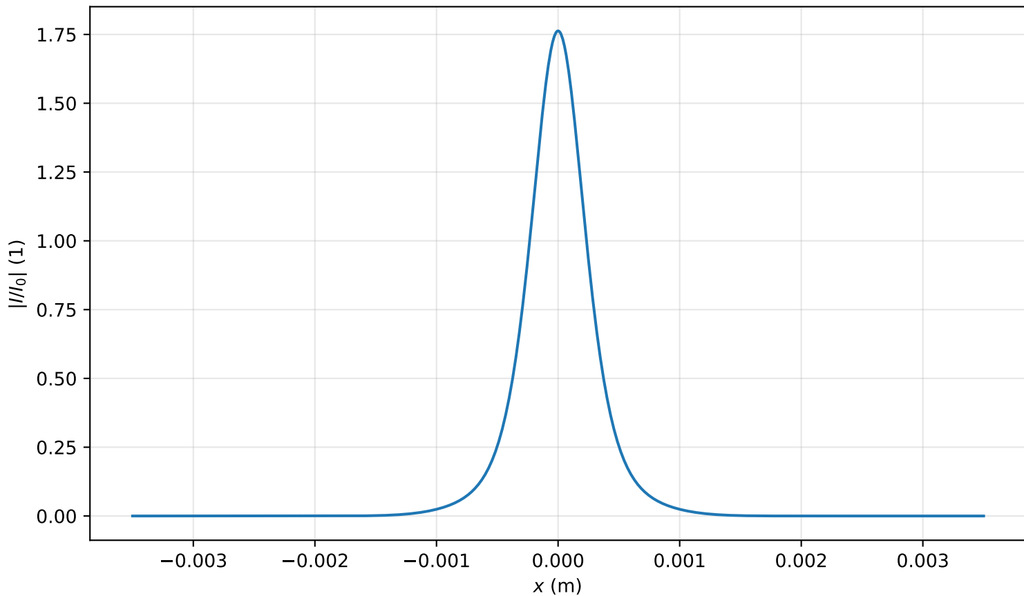
Intensity profile I(x, y = 0, z = 1.353m)/I_0 , P_{in}=1.0P_{cr} , artificial time
